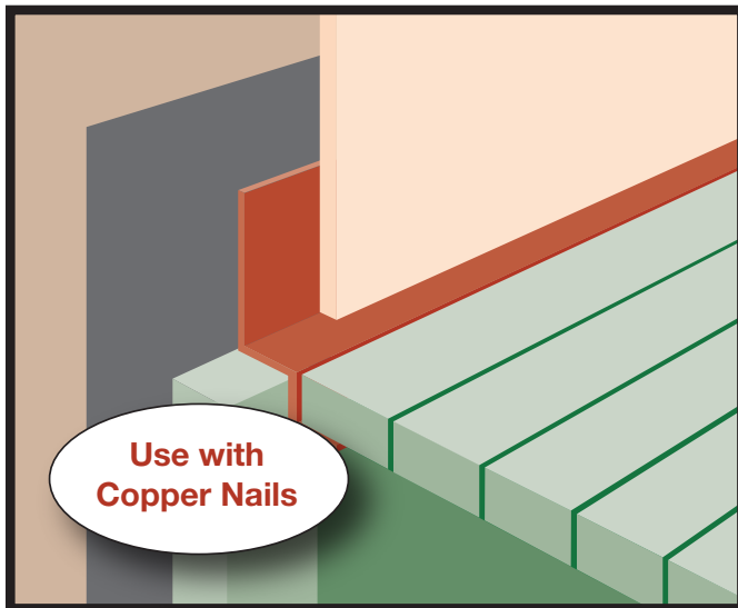
Use as a Ledger Flashing when working with ACQ Treated Lumber.
