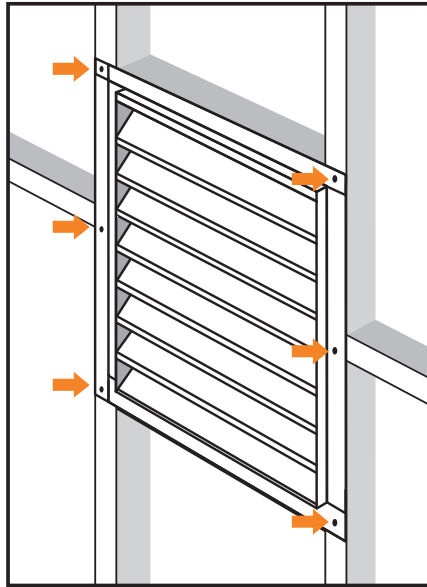
2) Insert vent into opening and fasten to frame with galvanized nails
