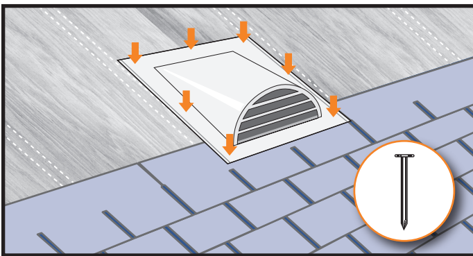
3. Center the throat of the vent over the roof opening. Fasten with 7 galvanized roofing nails. Note: Hem may be hammered flat by installer.
