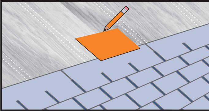
1. Make a template of the Rough Opening. Center the template between rafters on the rear slope of the house.
