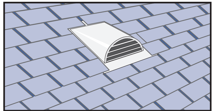
4. Finish installation by sealing all seams, nails and loose edges of shingles with roofing cement.
